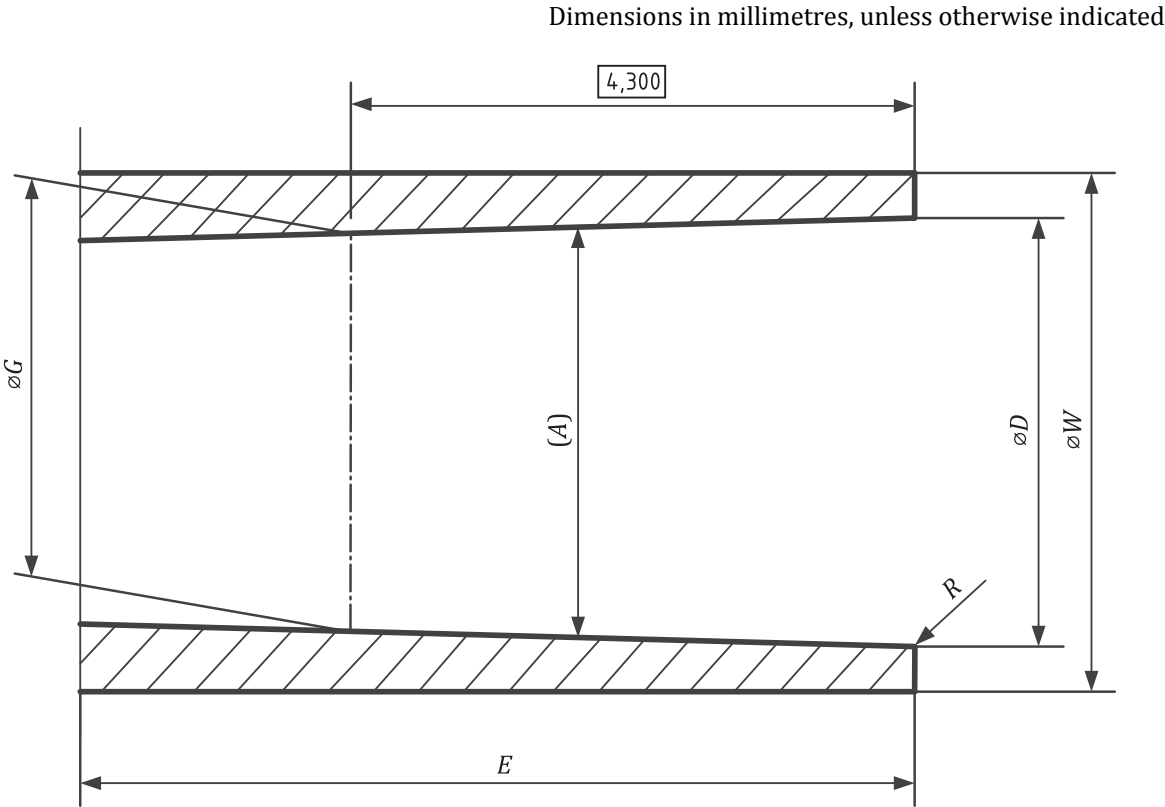
Figure EE.1 — Removable temperature sensor port
